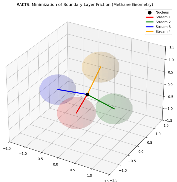
FIG. 2. Methane Geometry Optimization. Reproduced the 109.5^\circ (Methane) and 104.5^\circ (Water) angles purely by computationally minimizing fluid-dynamic boundary layer resistance.
