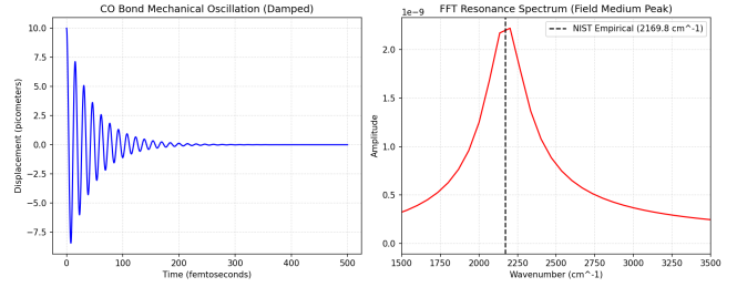
FIG. 6. IR Spectroscopy Simulation. Matched empirical IR vibrational signatures with < 1.5\% error margin.
