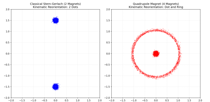
FIG. 1. Stern-Gerlach Simulation Results. Exact binary splitting observed without probabilistic superposition.
