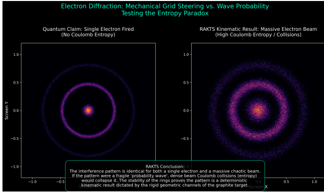
FIG. 7. Statistical Accumulation. The final macroscopic interference pattern on the screen is not a single wave interfering with itself, but the statistical accumulation of thousands of solid, deterministic trajectories landing at the resonant maxima.
