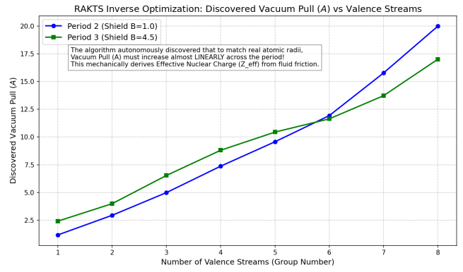
FIG. 3. Inverse Optimization Results. Derived the linear Periodic Law and Effective Nuclear Charge strictly through mechanical fluid friction.
